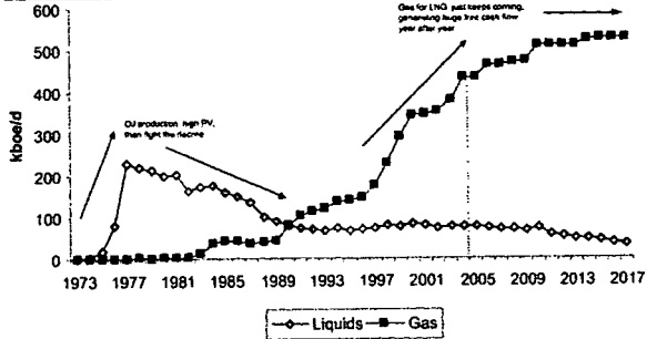
Figure 15: Example: oil and gas production at TOTAL's Bontang LNG plant
